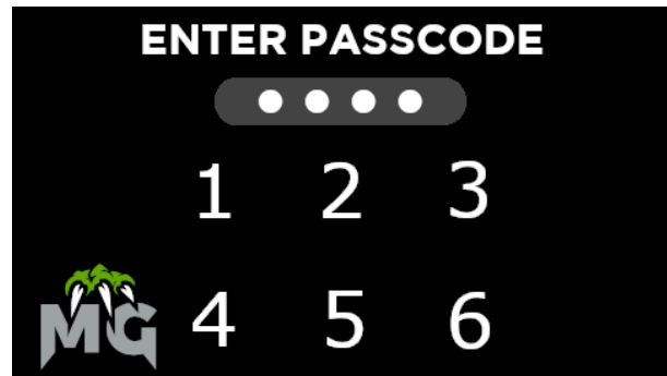
Lock Screen/Pass-code
